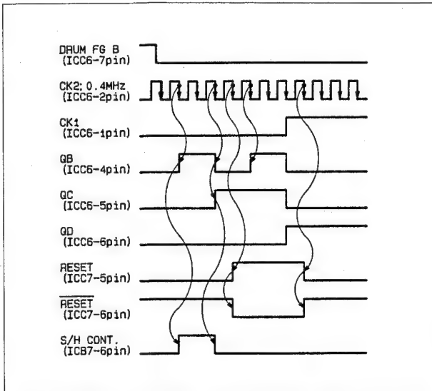
Fig. 4-3-4. Sample/hold Timing (CD-35 Board)
